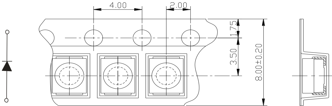
单位: mm, 未注公差: \pm 0.1 mm All dimensions in mm, tolerances unless mentioned is \pm 0.1 mm.
