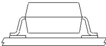
6LSOP-P type
