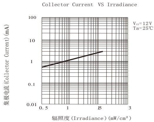
Collector Current VS Irradiance
