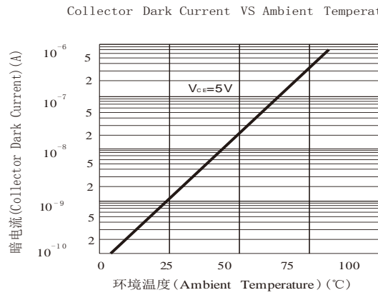
Collector Dark Current VS Ambient Temperature
