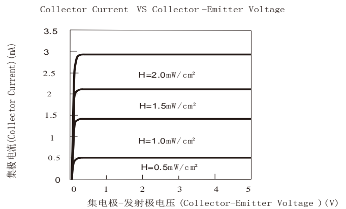
Collector Current VS Collector-Emitter Voltage
