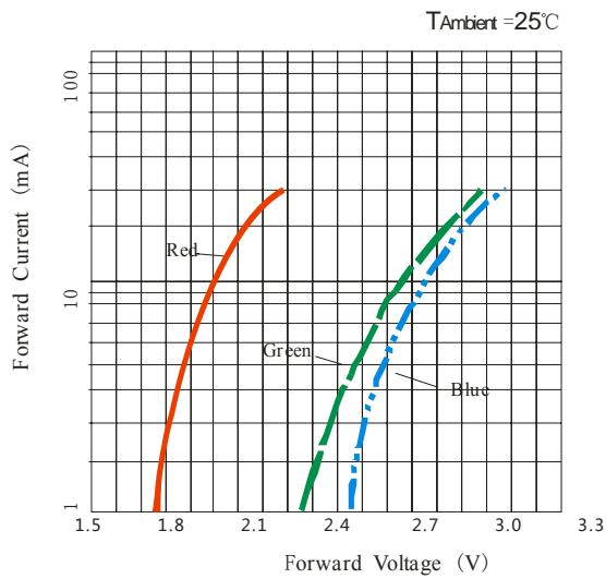
Volt-Ampere Characteristics
