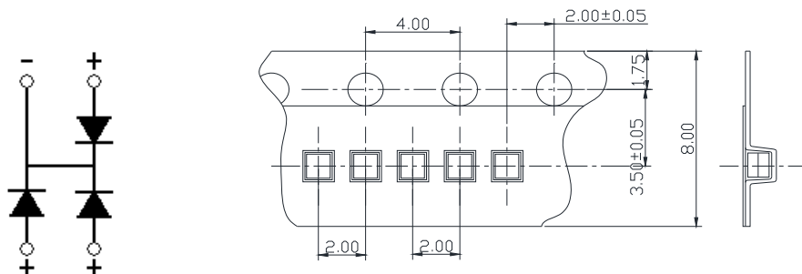
单位: mm, 未注公差: \pm 0.1 mm All dimensions in mm, tolerances unless mentioned is \pm 0.1 mm.
